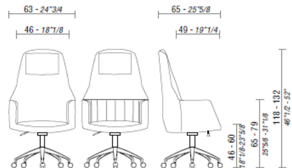
TULIP, chair with high backrest.
