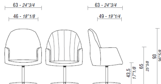
TULIP, chair with cross-shaped base and medium backrest.
