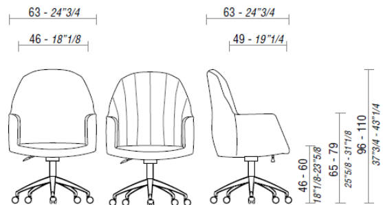
TULIP, chair with medium backrest.
